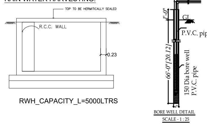
BORE WELL DETAIL SCALE - 1:25
