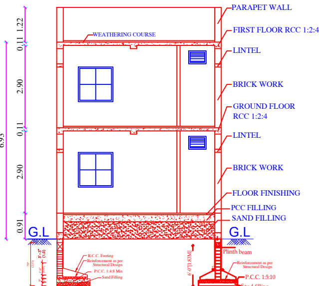
CROSS SECTION ON A-A
