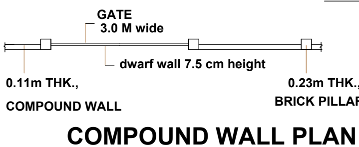
COMPOUND WALL PLAN
