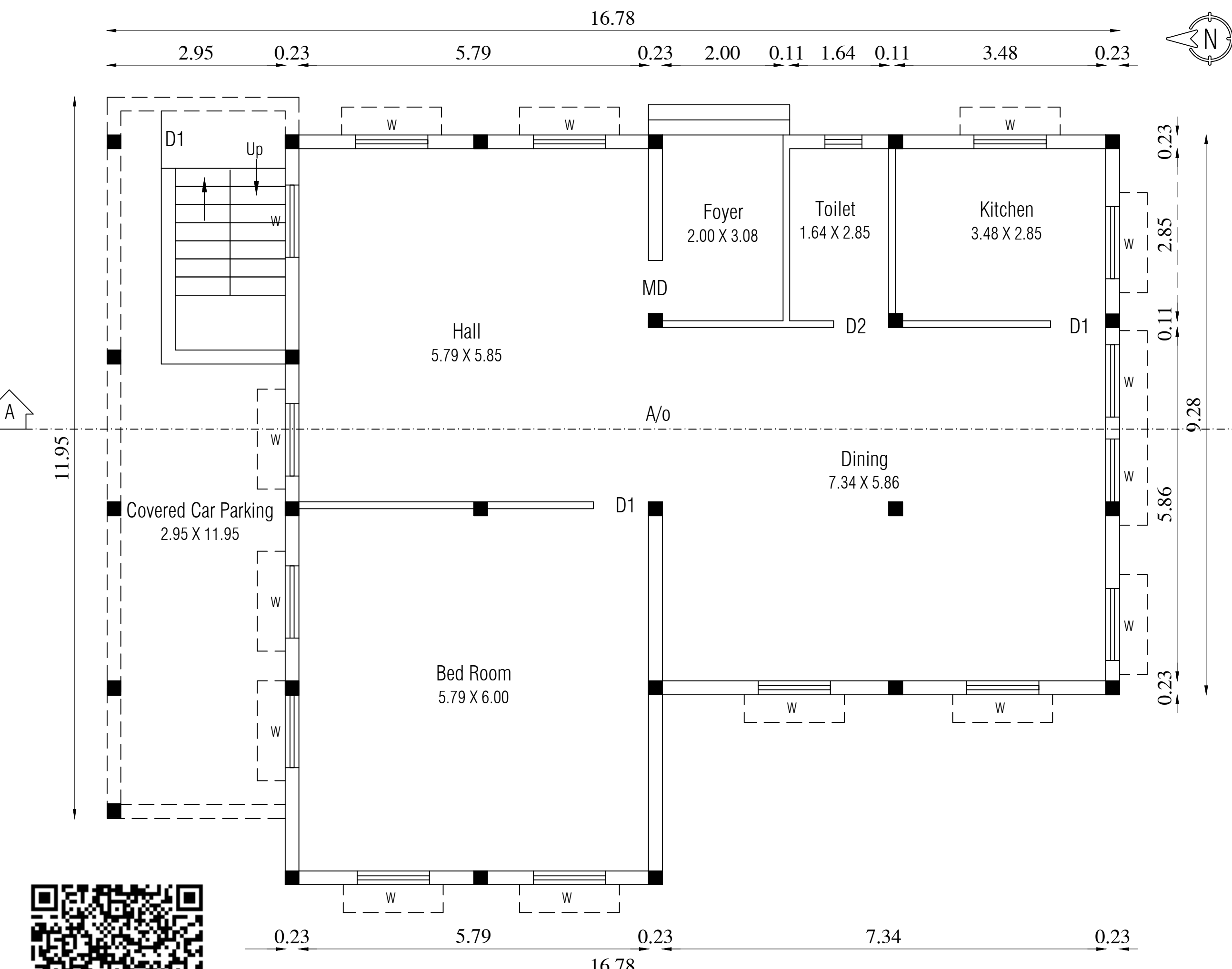
Pro.Ground Floor Plan
