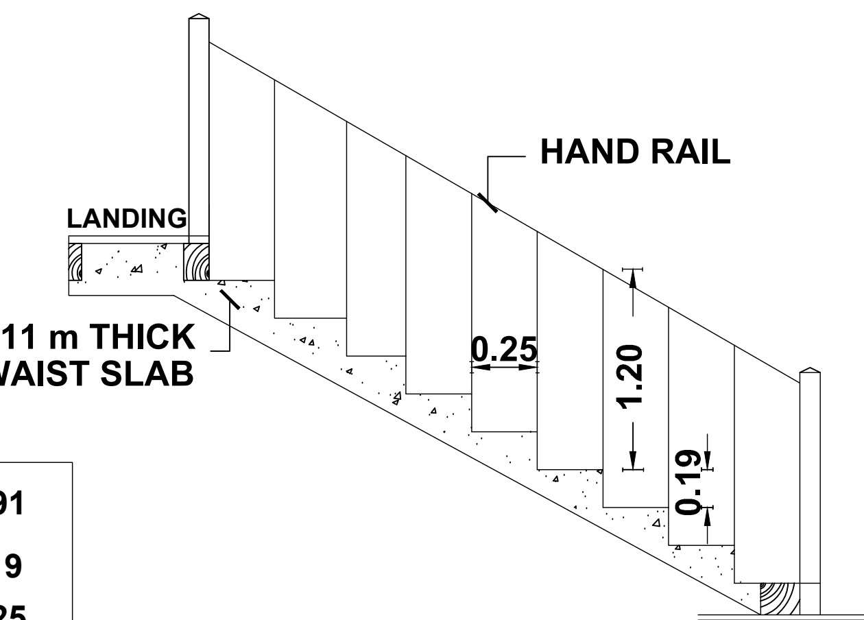
STAIRCASE DETAIL
