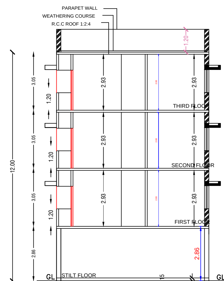
SECTION ON AB (PROPOSED)
