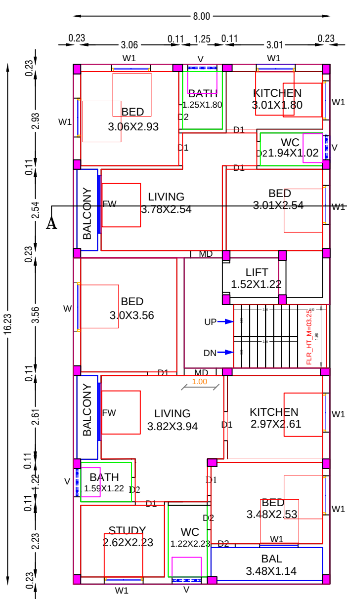
THIRD FLOOR PLAN (PROPOSED)
