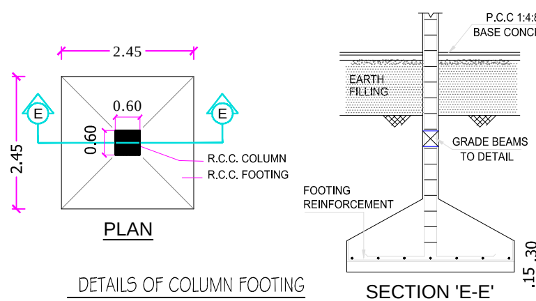
DETAILS OF COLUMN FOOTING
