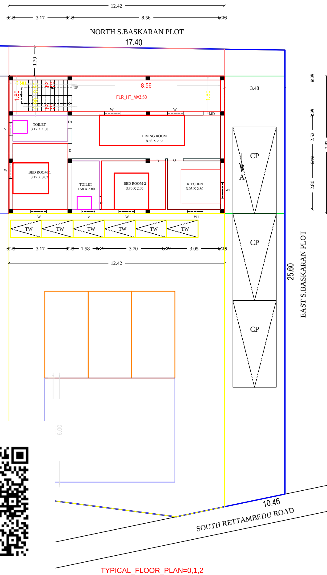
SITE/PROPOSED GROUND FLOOR PLAN
