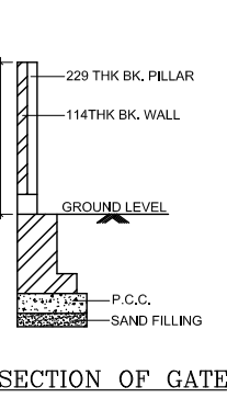
SECTION OF GATE
