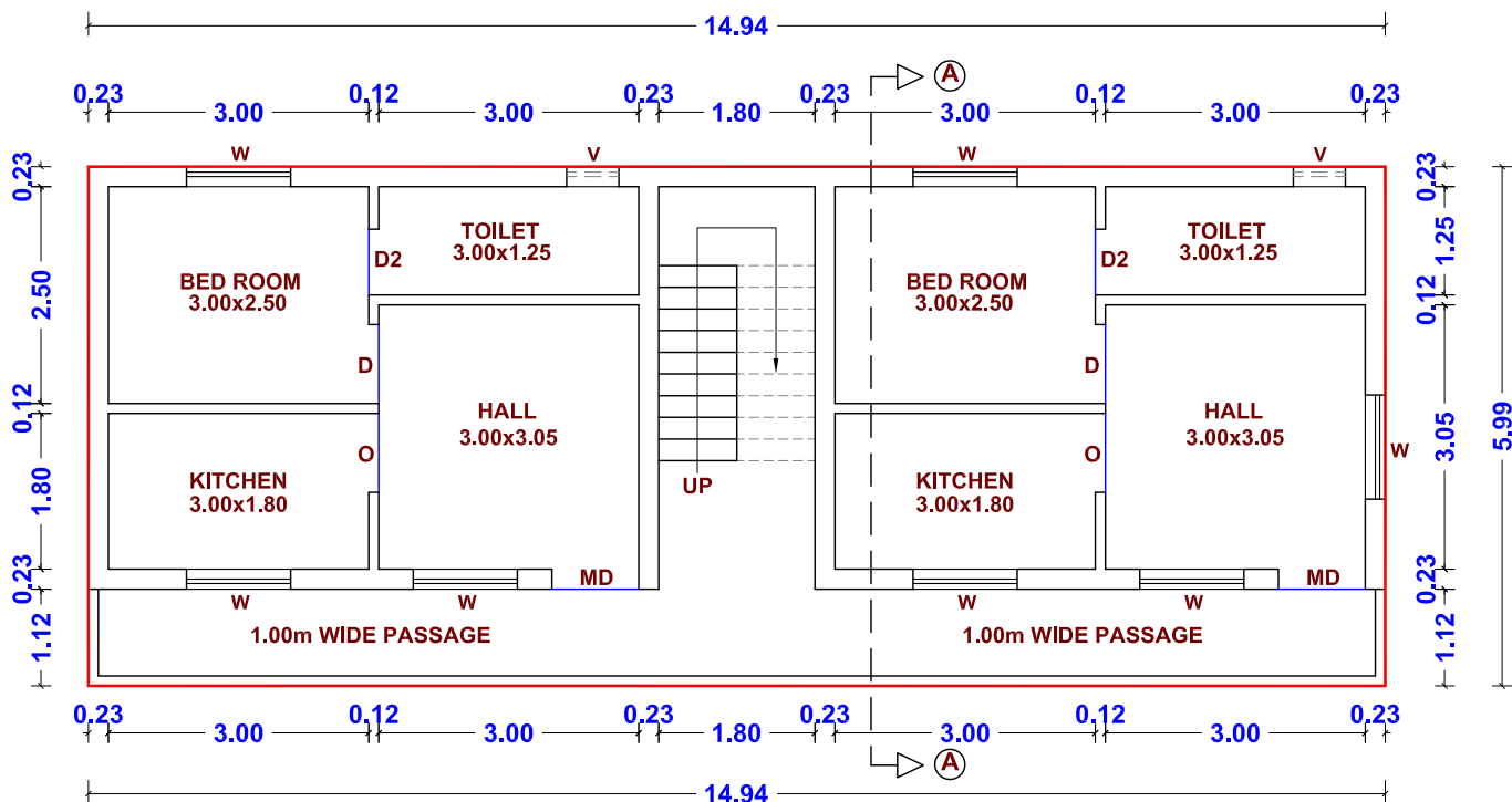
TYPICAL 1st & 2nd FLOOR PLAN
