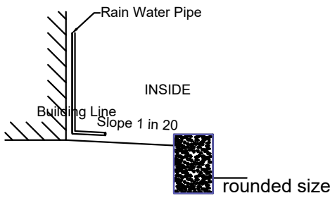
RAINWATER HARVESTING
