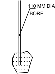
BOREWELL
