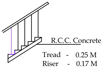
Staircase details
