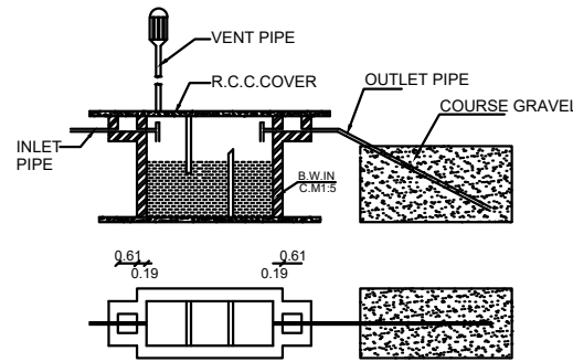
SEPTIC TANK & DISPERSION TRENCH DETAILS
