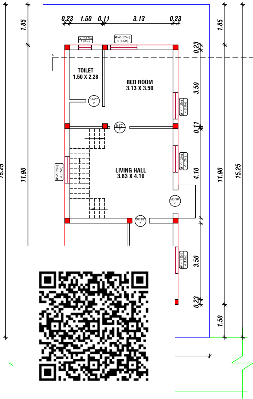
SITE CUM PRO.GROUND FLOOR PLAN
