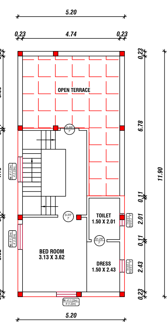
PRO.SECOND FLOOR PLAN WITH OPEN TERRACE
