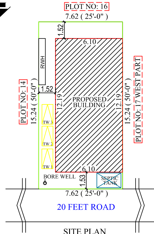
SITE PLAN
