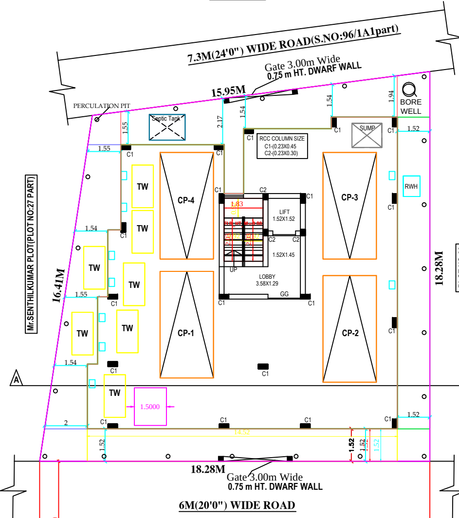
FLOOR PLAN PROPOSED
