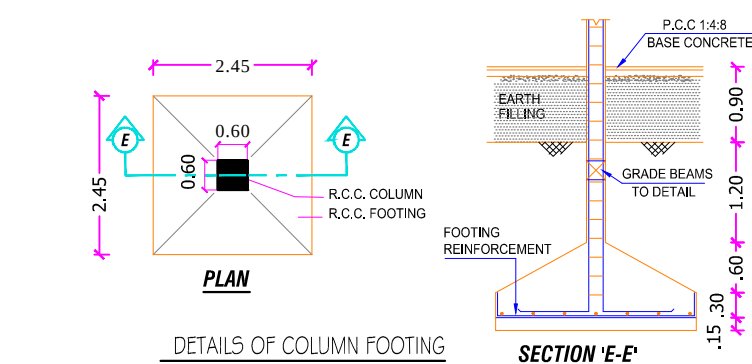
DETAILS OF COLUMN FOOTING
