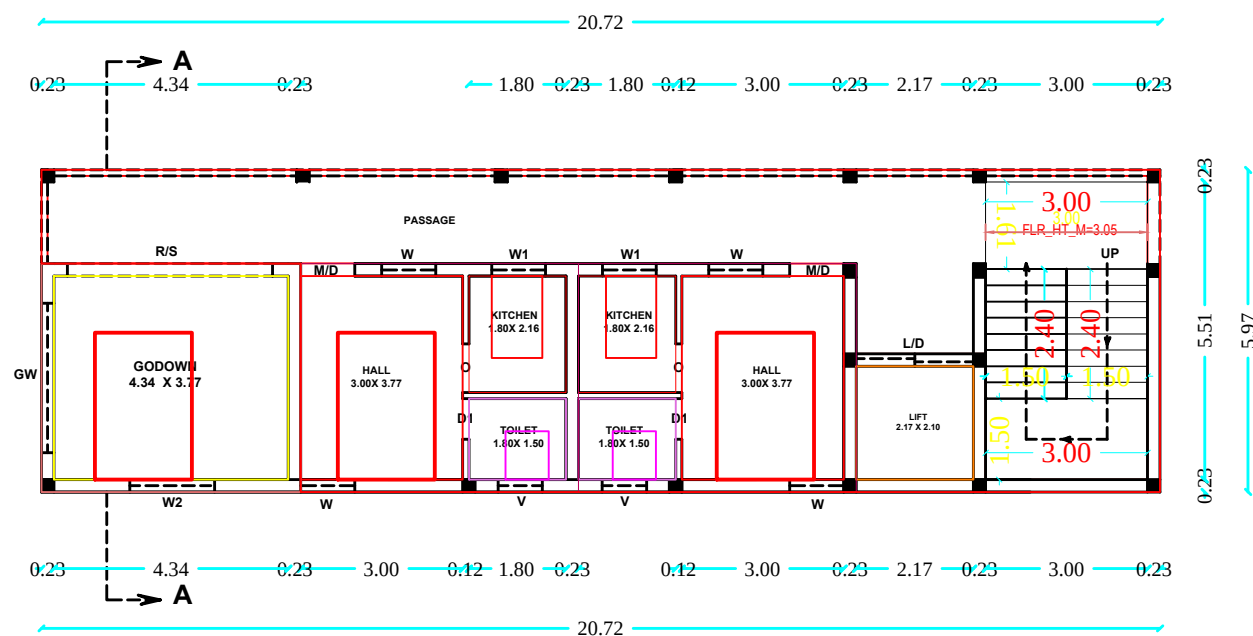
FIRSAT FLOOR PLAN
