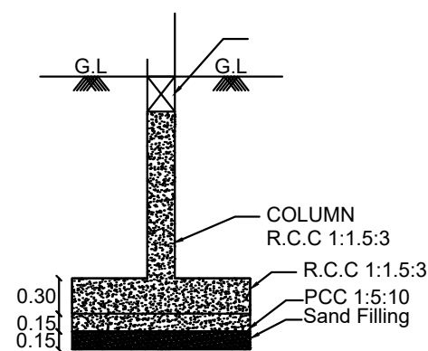
Foundation Details
