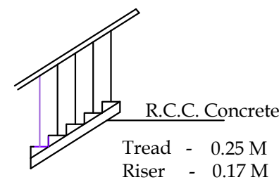
Staircase details
