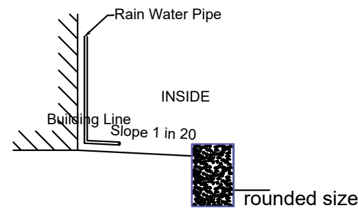
RAINWATER HARVESTING
