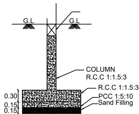
Foundation Details
