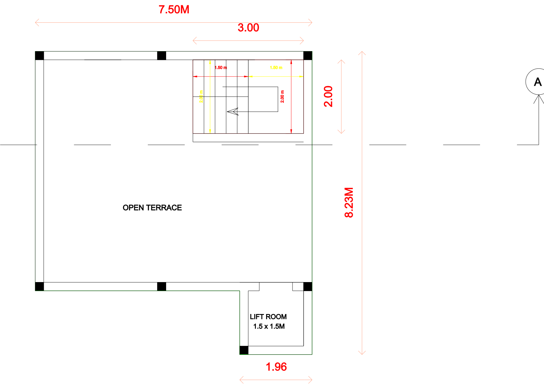
TERRACE FLOOR PLAN 1:100
