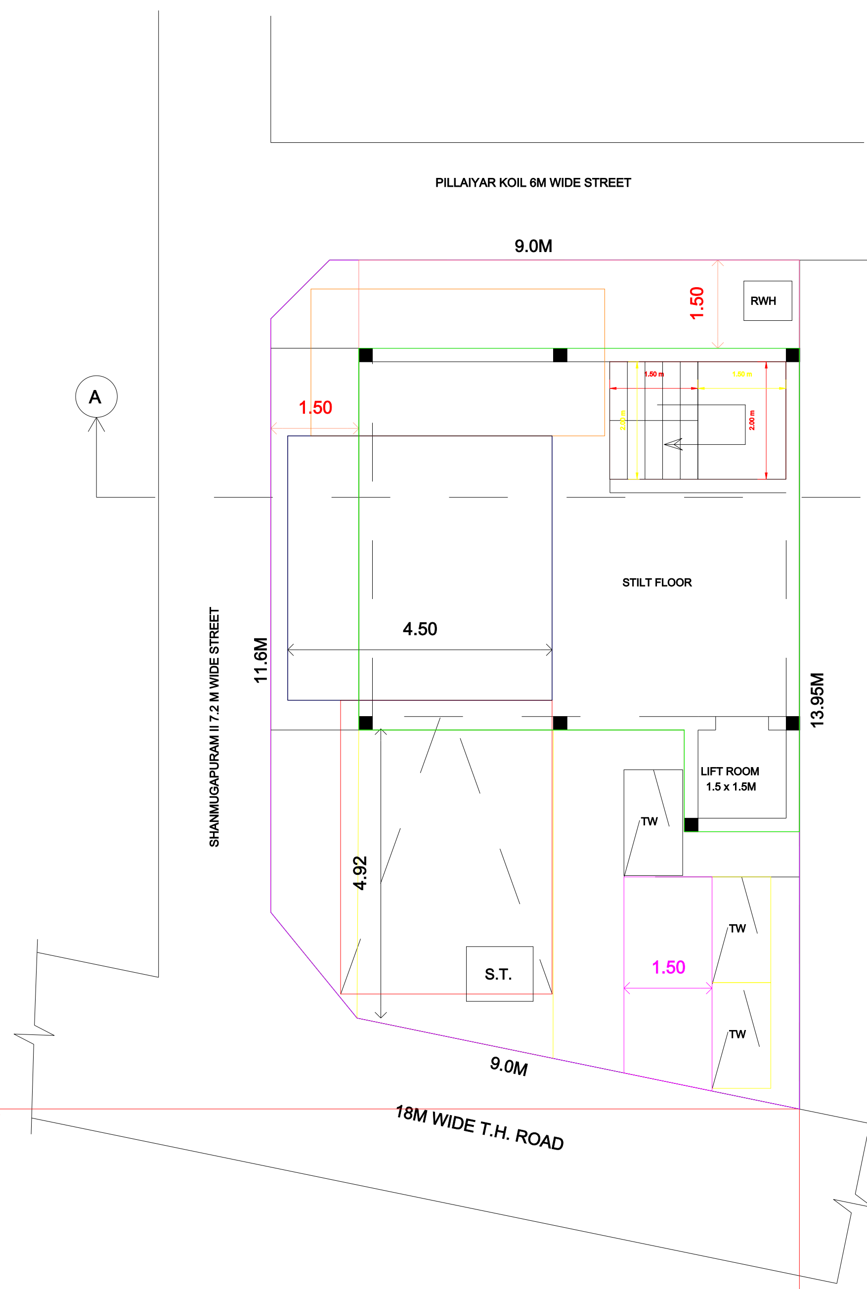
TE CUM STILT FLOOR PLAN 1:100
