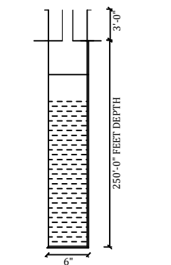
BORE DETAILS
