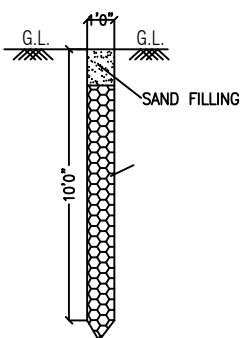
PERCOLATION PIT DETAILS
