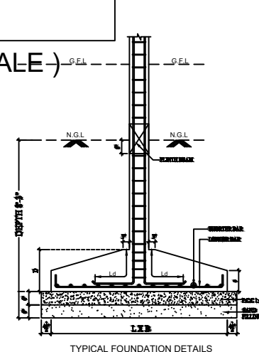
TYPICAL FOUNDATION DETAILS
