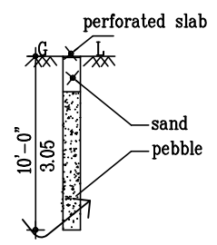
Rain Water Percolation Pits @ 3mc/c
