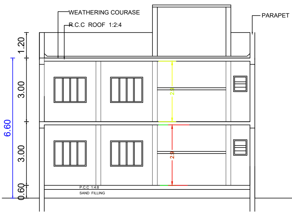
SECTION ON A - A (PROPOSED)
