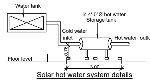
Solar hot water system details
