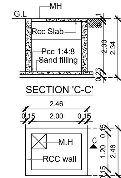
PLAN DRINKING WATER SUMP (Scientifically Closed)
