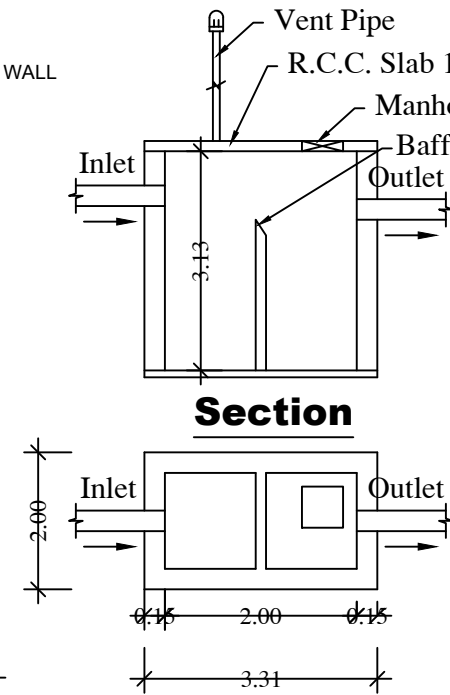
Plan Details of Septic Tank
