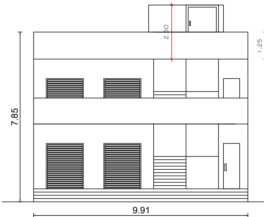
ELEVATION (PROPOSED)
