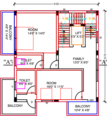
TYPICAL_FLOOR_PLAN=2,3,4
