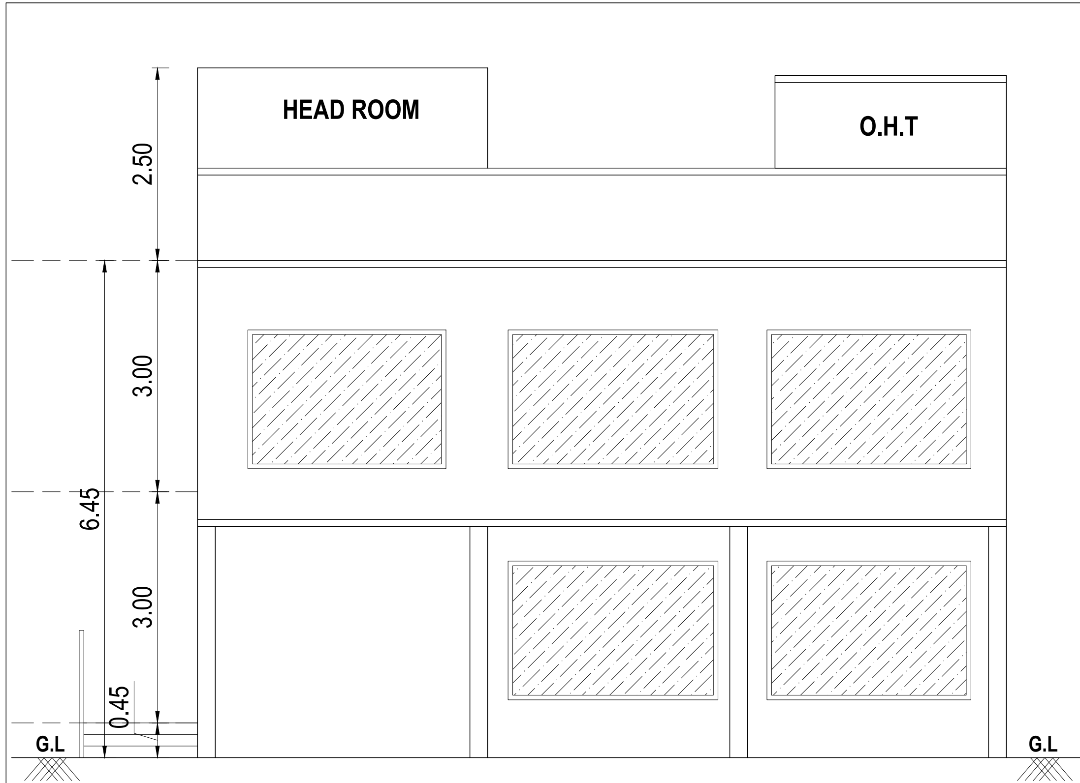
FRONT ELEVATION
