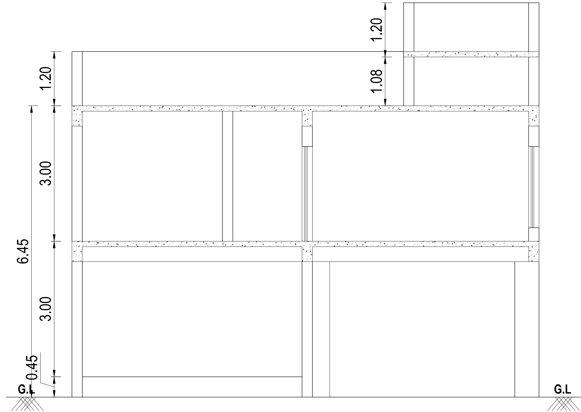
SECTION-A-A'
