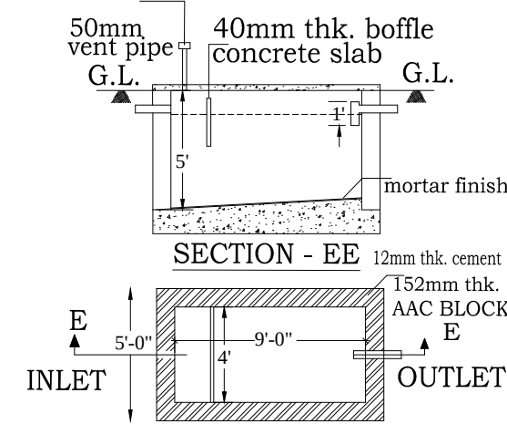
PLAN DETAILS OF SEPTIC TANK DETAILS OF SEPTIC TANK
