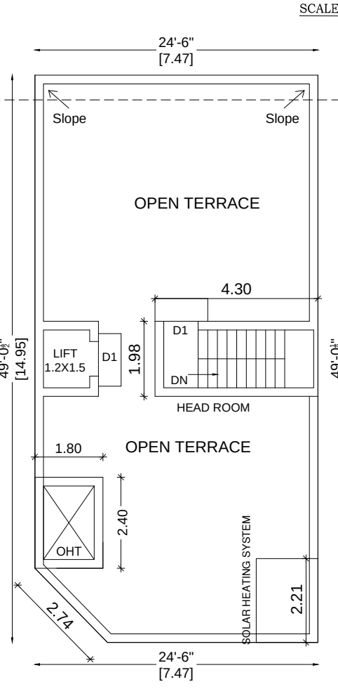
OPEN TERRACE FLOOR PLAN
