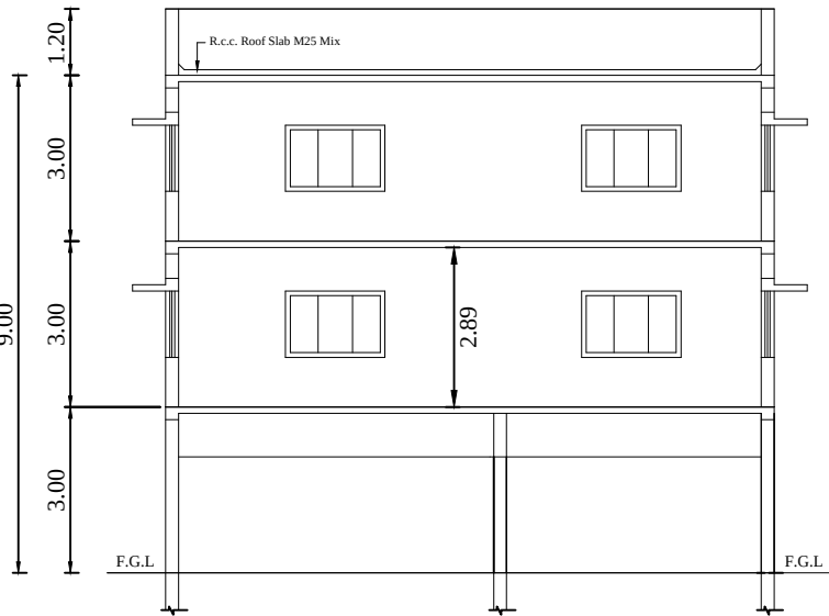
SECTION ON A - A [ PROPOSED ]
