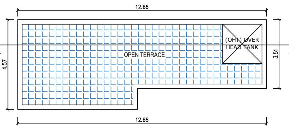
TERRACE FLOOR
