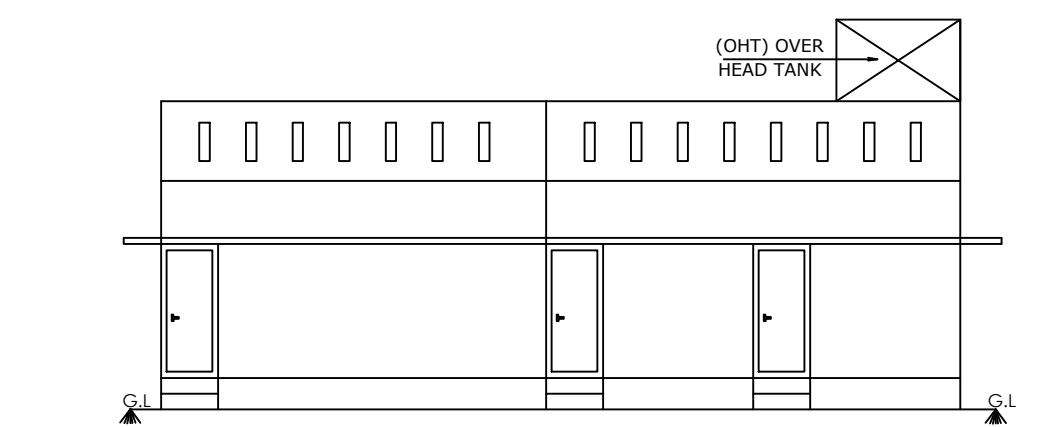
FRONT ELEVATION
