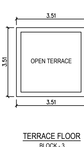
BLOCK - 3
