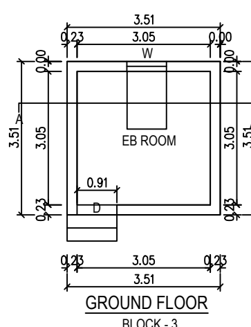
BLOCK - 3
