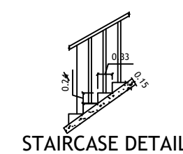
STAIRCASE DETAIL
