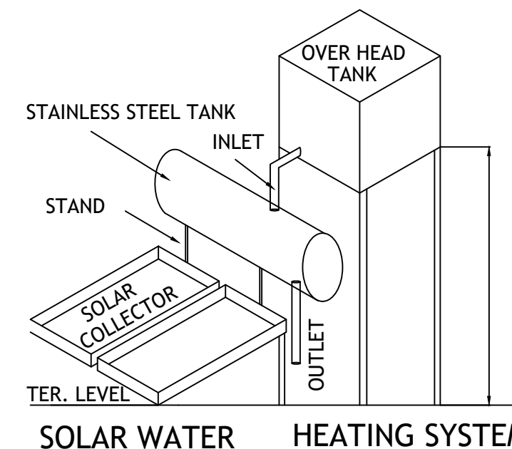
SOLAR WATER
