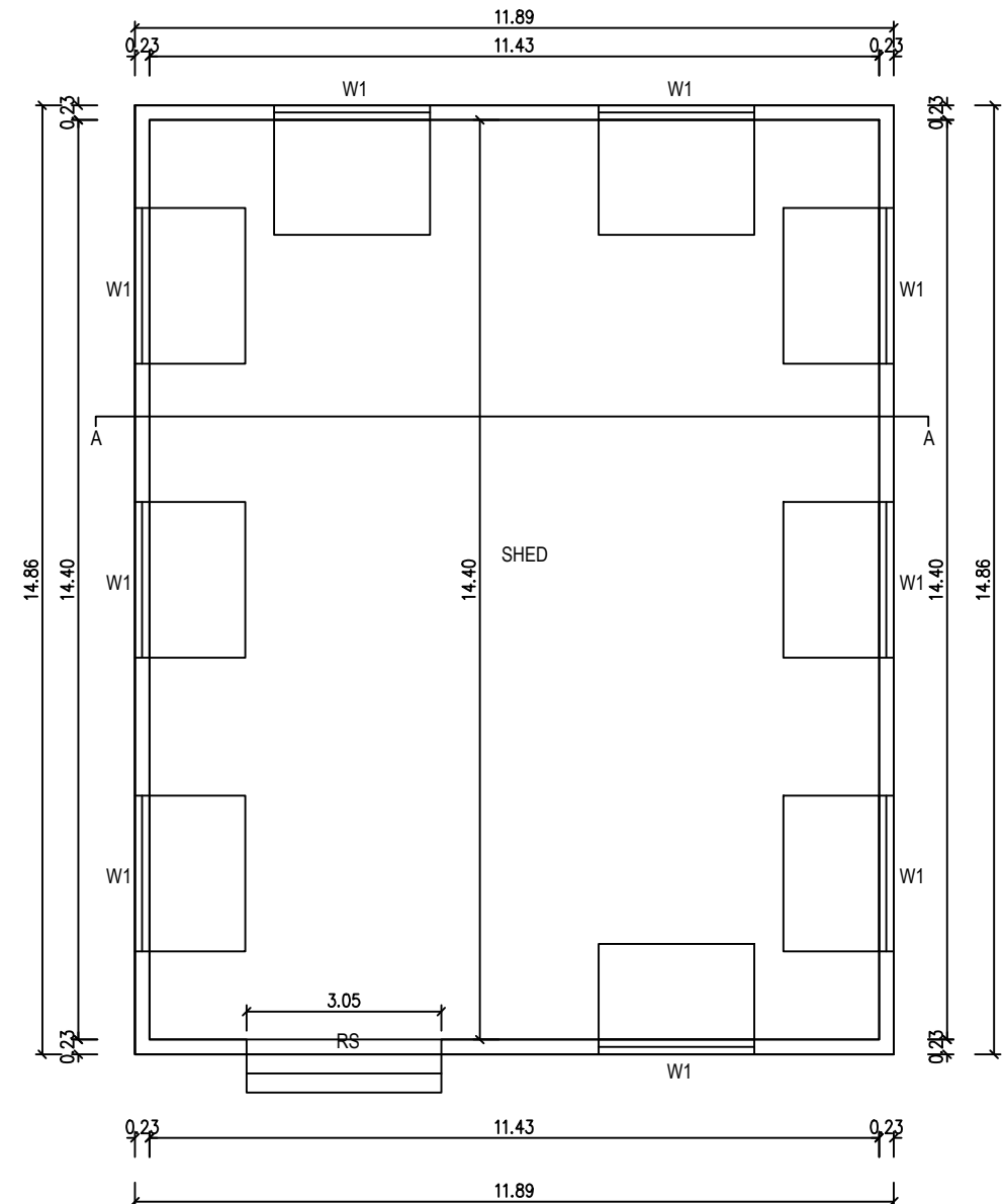
GROUND FLOOR
