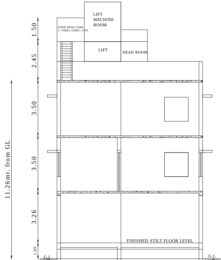
SECTION ON "AB" (PROPOSED)
