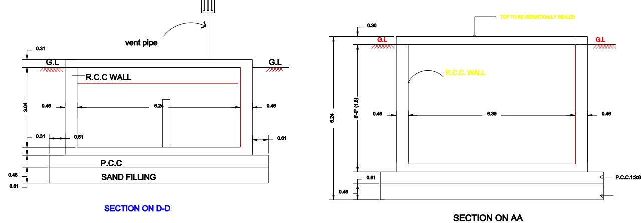
SECTION ON D-D
