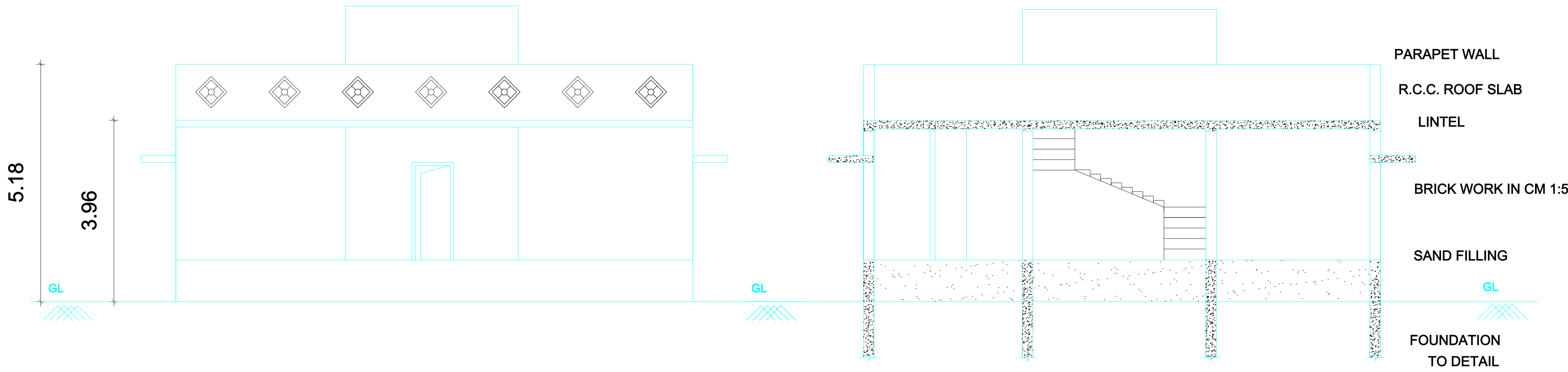
FRONT ELEVATION
