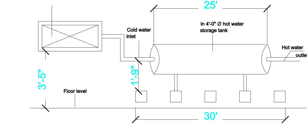
SOLAR HOT WATER SYSTEM(SWHS) DETAIL
