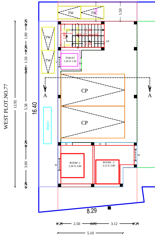
SITE/PROPOSED GROUND FLOOR PLAN
