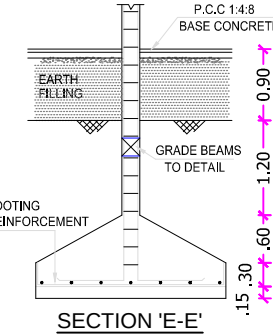
SECTION 'E-E'
