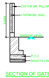
SECTION OF GATE
