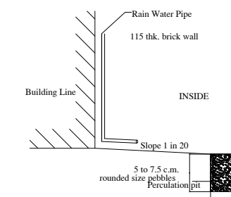
PERCOLATION PIT
