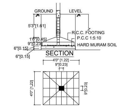
FOUNDATION DETAILS
