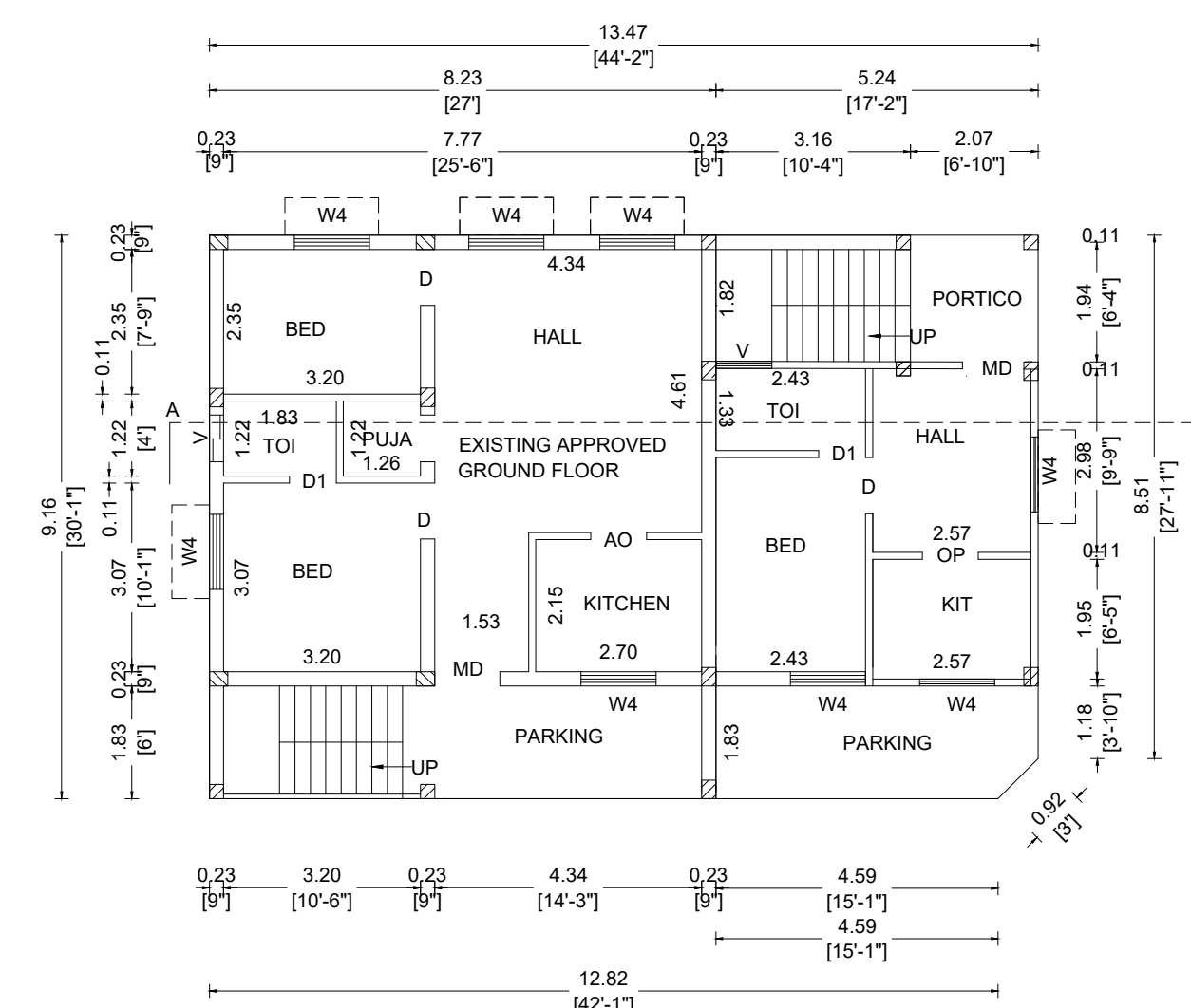
[42'-1"] EXISTING APPROVED GROUND FLOOR PLAN & PROPOSED ADDITIONAL GROUND FLOOR PLAN
