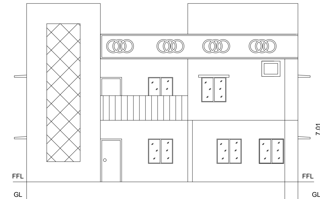
SOUTH ELEVATION (PROPOSED)
