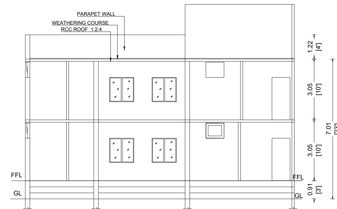
SECTION -AA' (PROPOSED)
