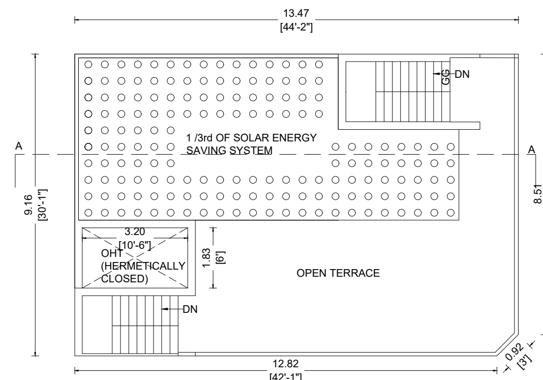
[42-1] TERRACE PLAN (PROPOSED)
