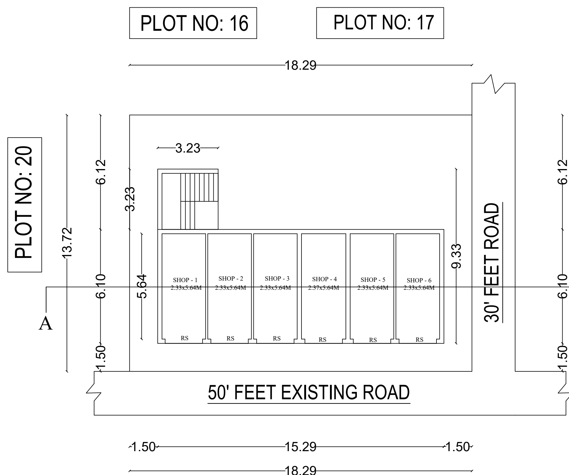
SITE CUM GROUND FLOOR
