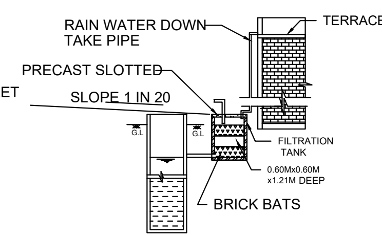
RAIN WATER HARVESTING SYSTEM
