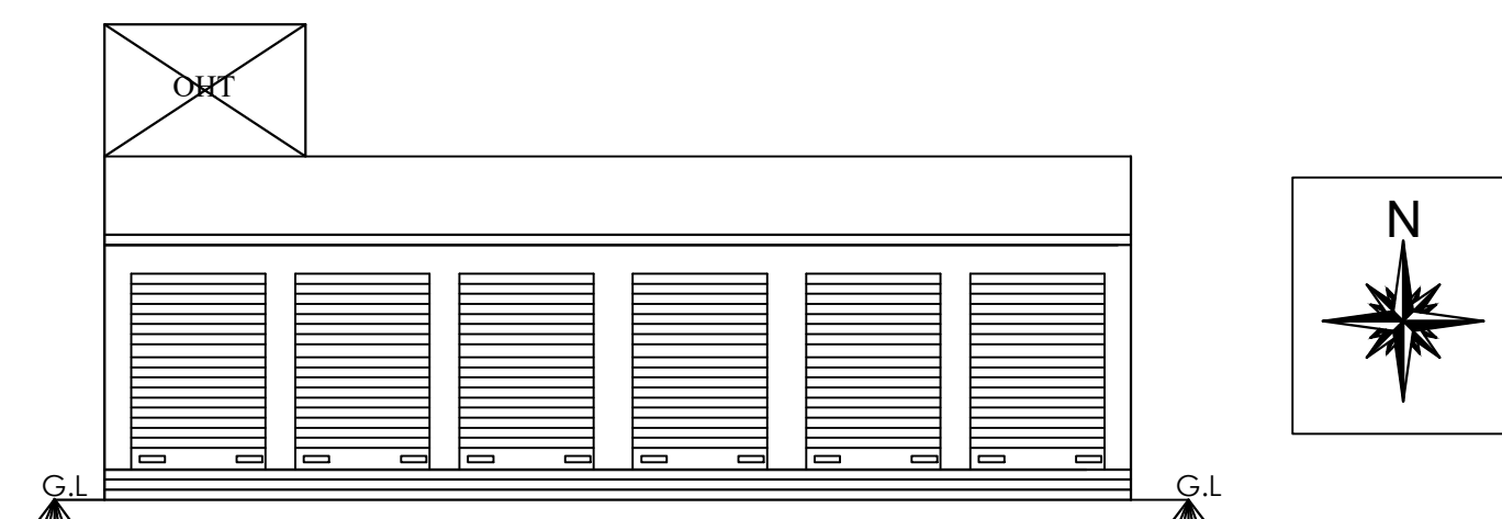
FRONT ELEVATION
