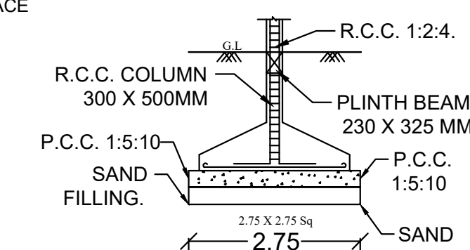
FOUNDATION DETAIL
