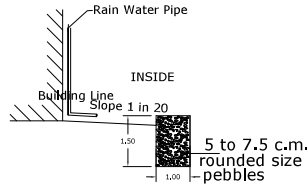
RAINWATER HARVESTING
