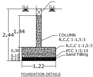
FOUNDATION DETAILS
