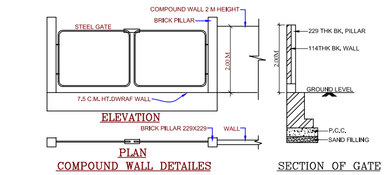
SECTION OF GATE
