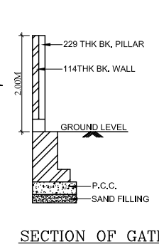
SECTION OF GATE
