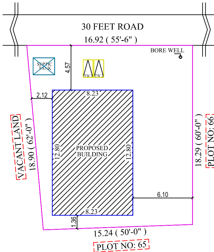
SITE PLAN
