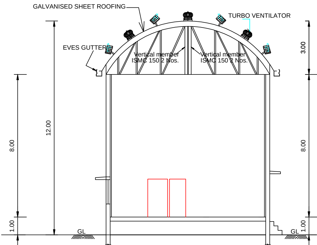
SECTION ON "AA" (PROPOSED)
