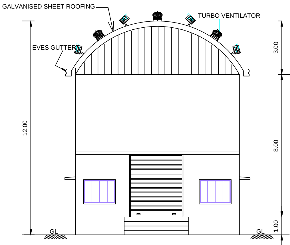
FRONT ELEVATION (PROPOSED)
