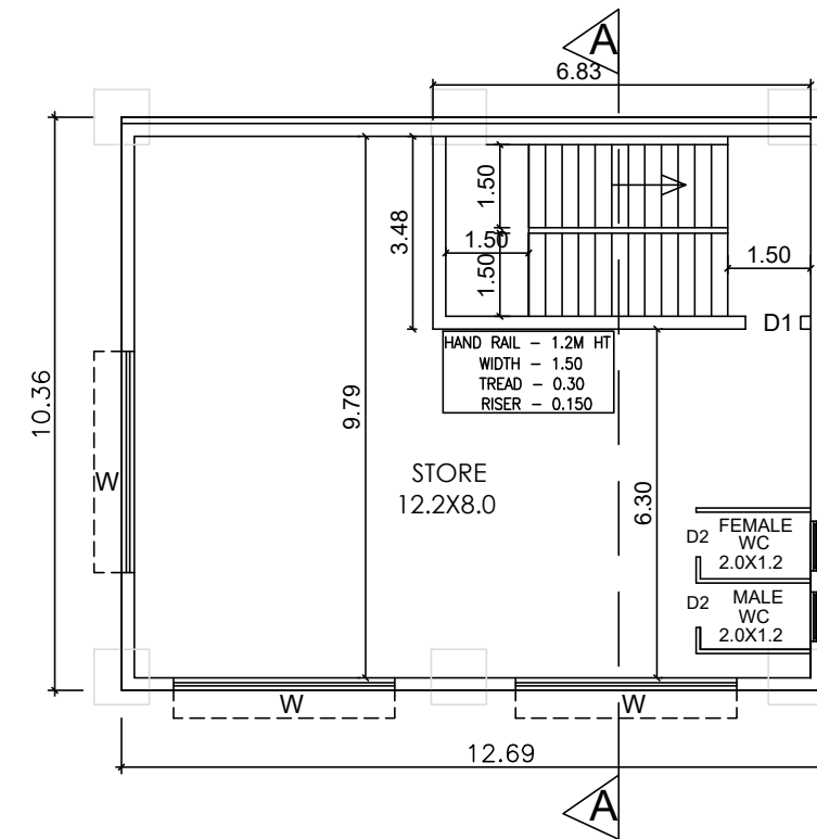
MEZZANINE FLOOR PLAN STORE ROOM
