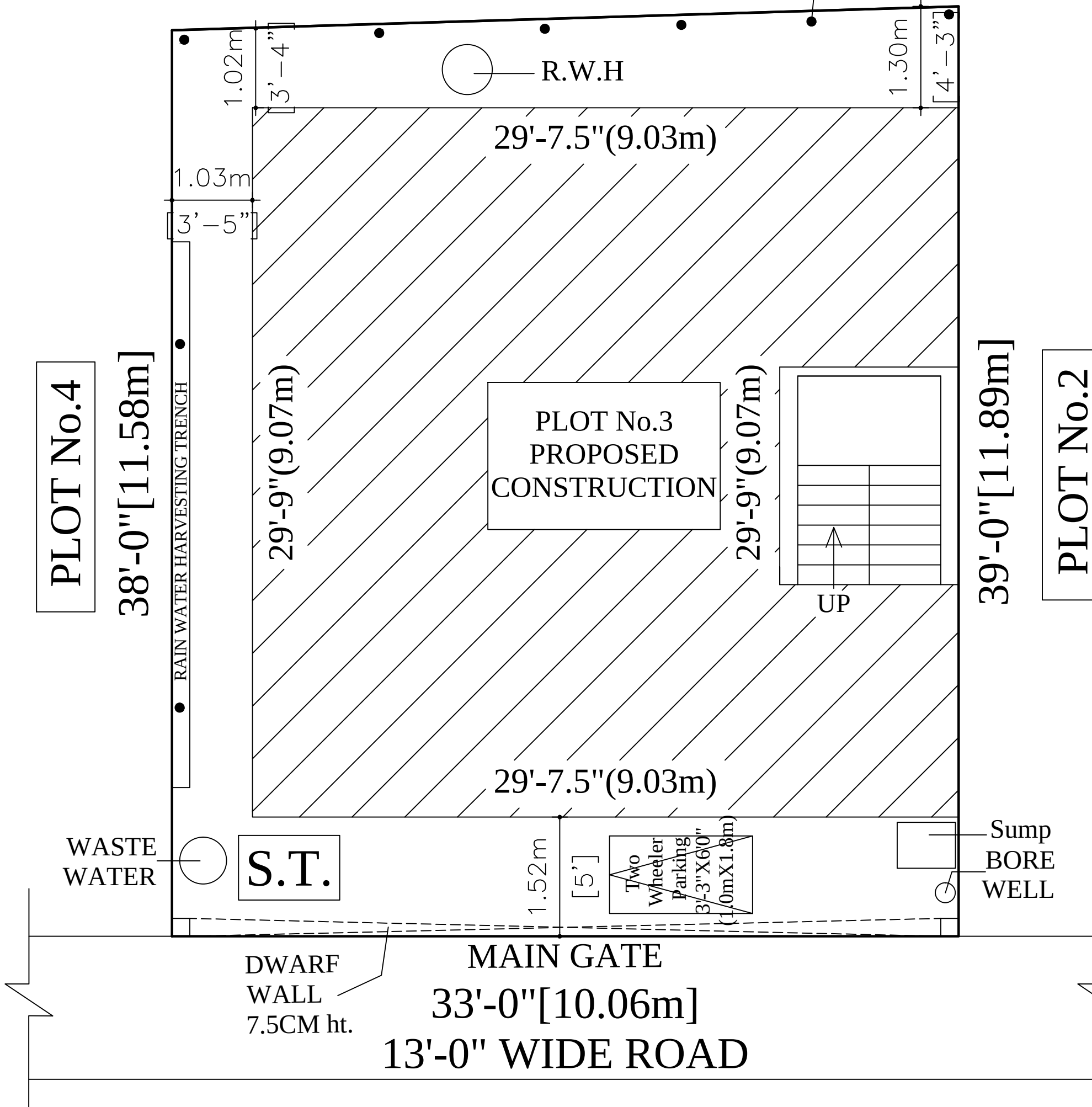
SITE PLAN
