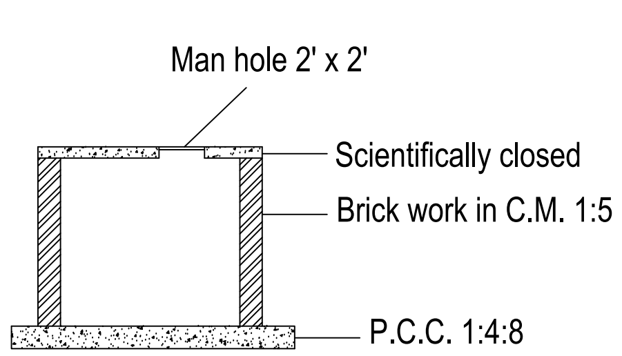
SECTION
