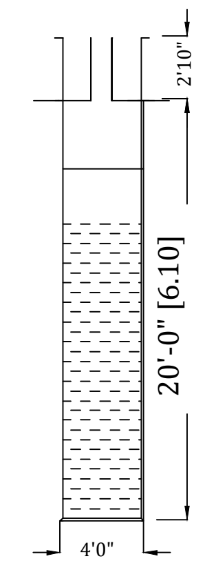
WELL DETAILS
