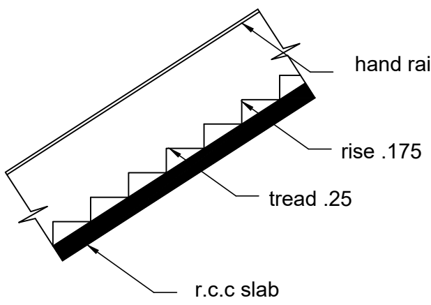
STAIR
