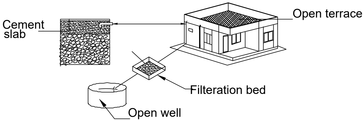
RAIN WATER HARVESTING
