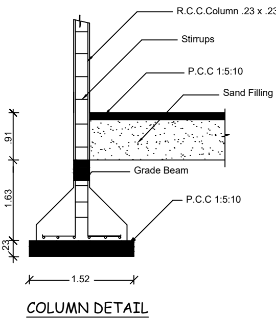
COLUMN DETAIL
