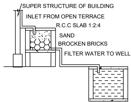
RAINWATER HARVESTING
