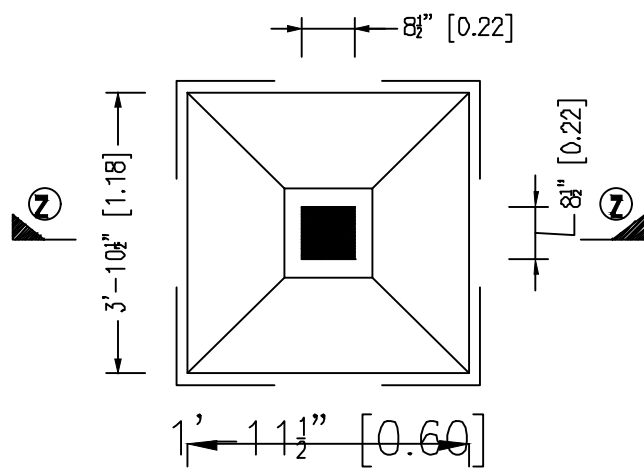
PLAN R.C.C COLUMN DETAILS
