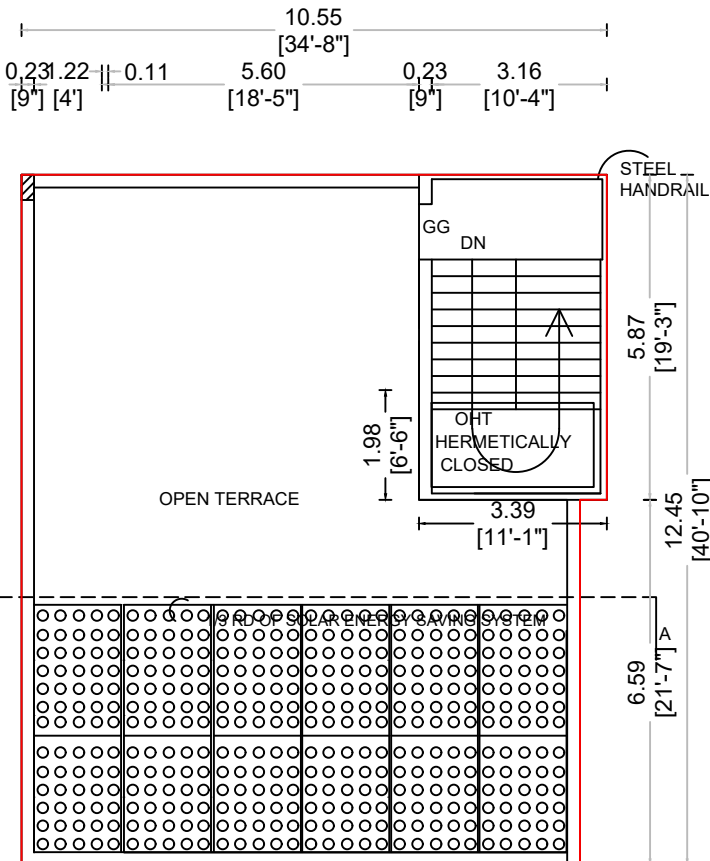
SECOND FLOOR PARTLY AND TERRACE FLOOR PLAN (PROPOSED)
