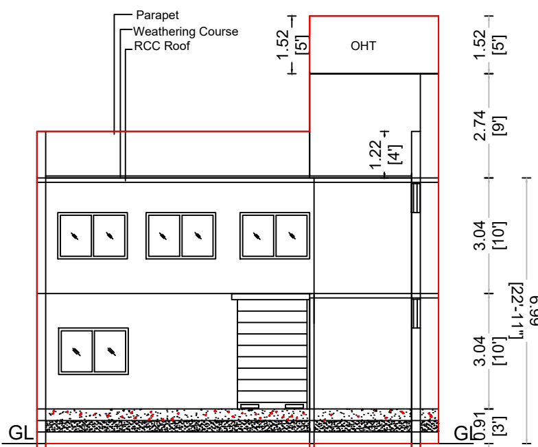
SECTION ON AA (PROPOSED)
