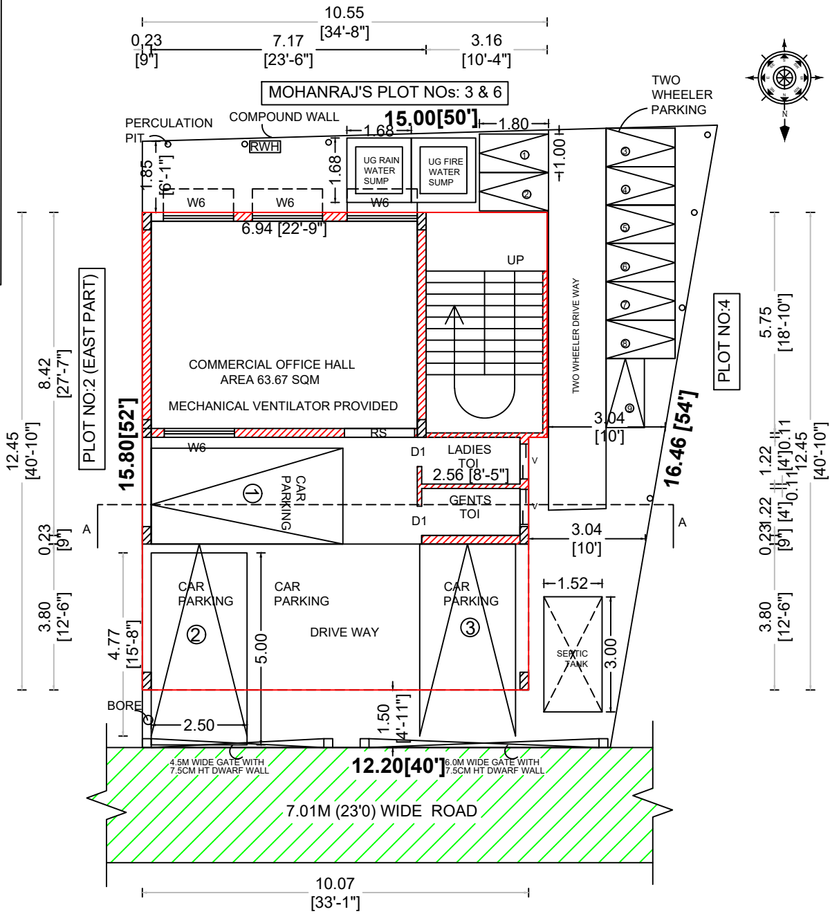
SITE CUM GROUND FLOOR PLAN (PROPOSED)
