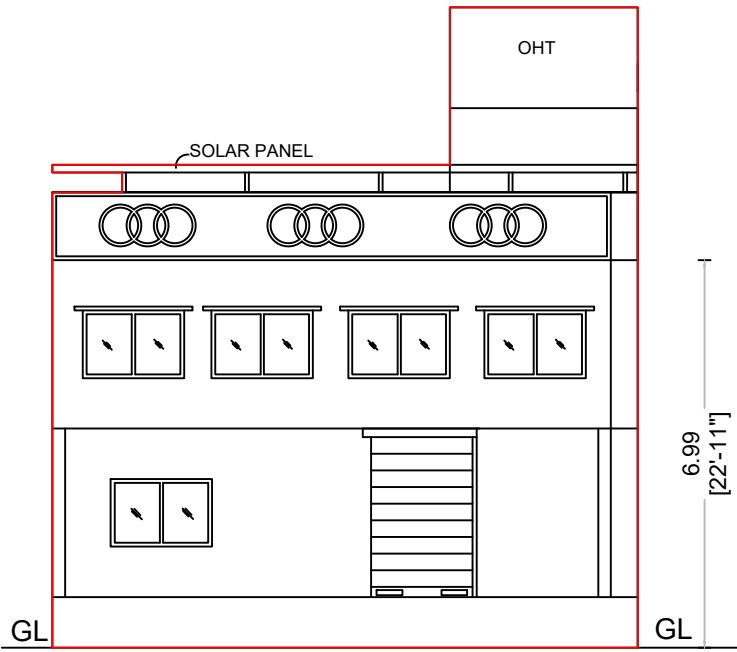
ELEVATION (PROPOSED)
