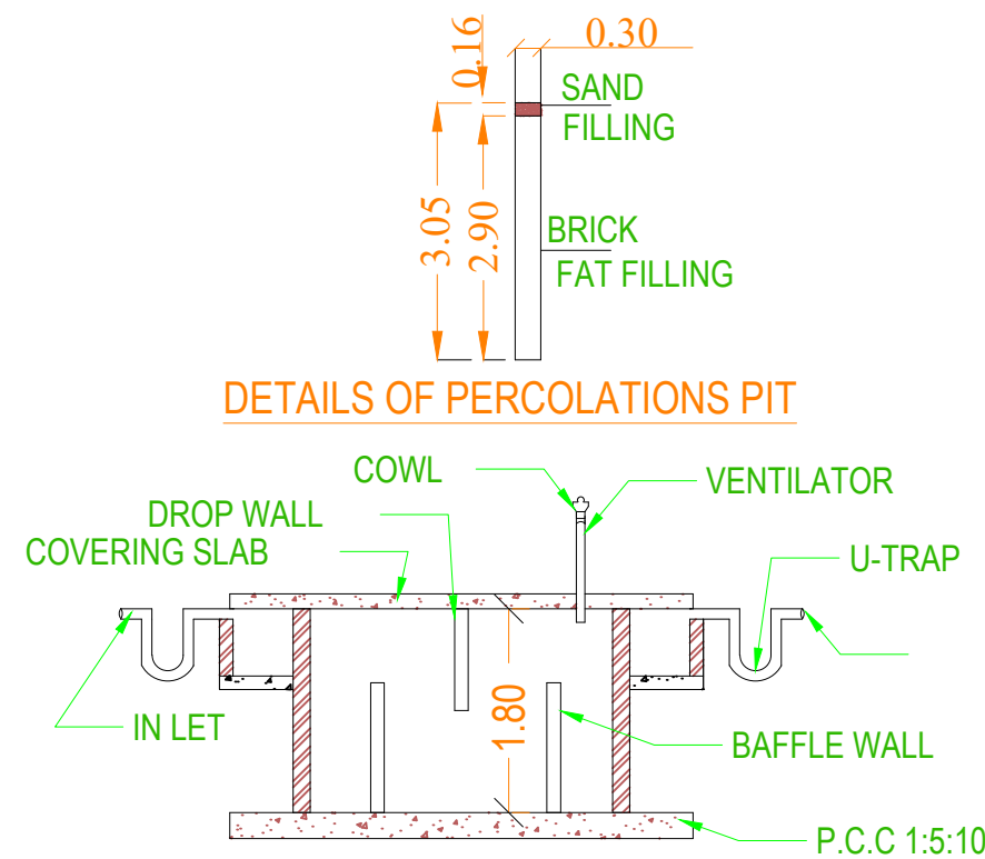
SECTION ON 'XY'
