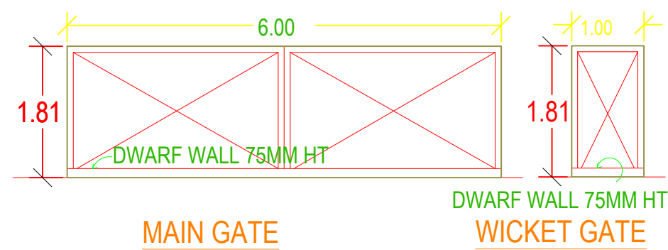
MAIN GATE
