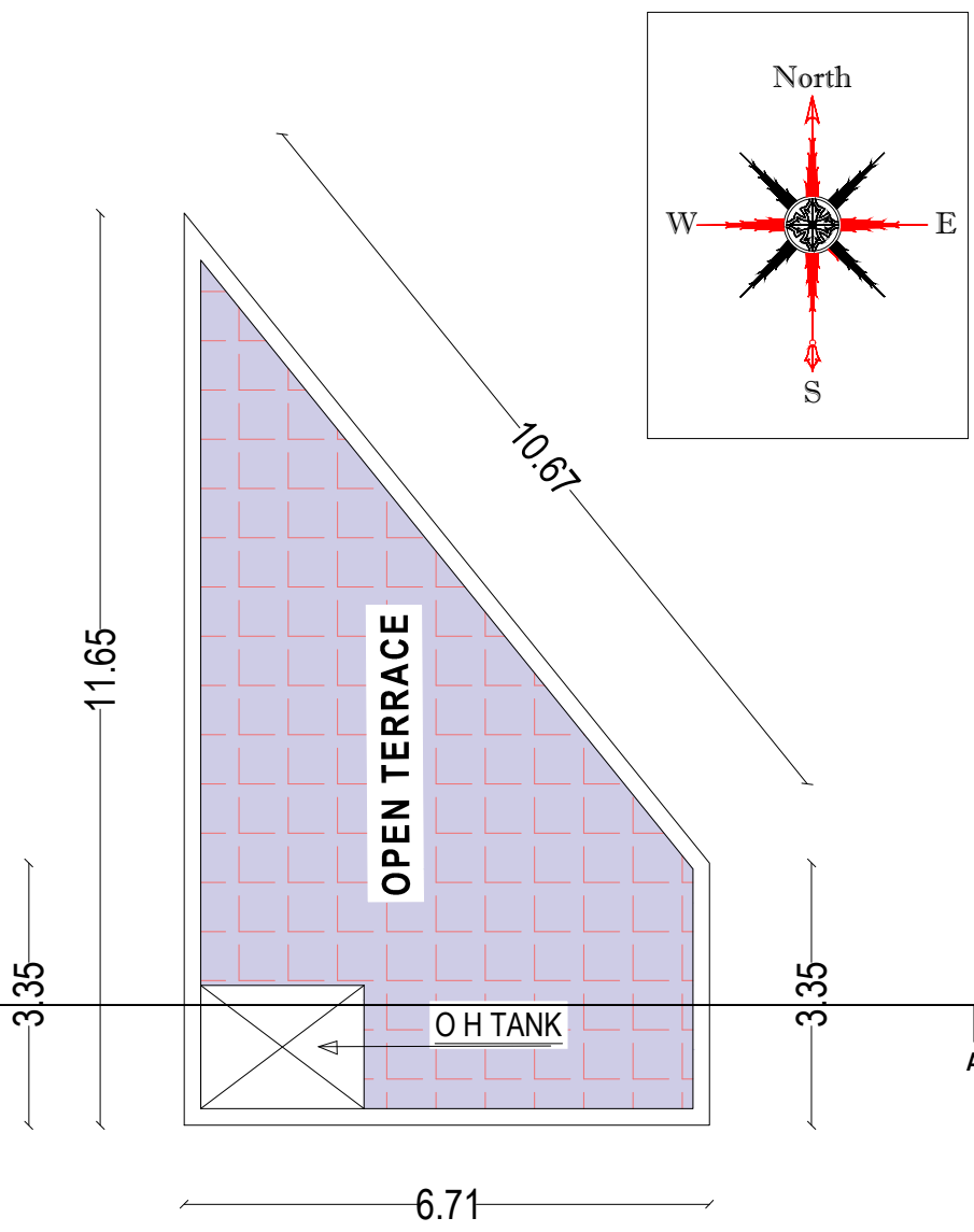
TERRACE FLOOR
