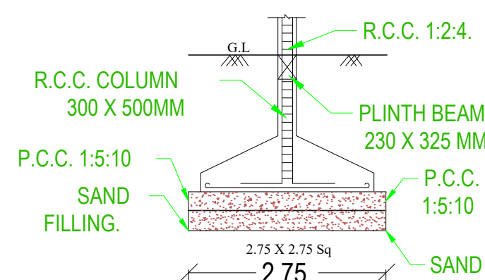
FOUNDATION DETAIL
