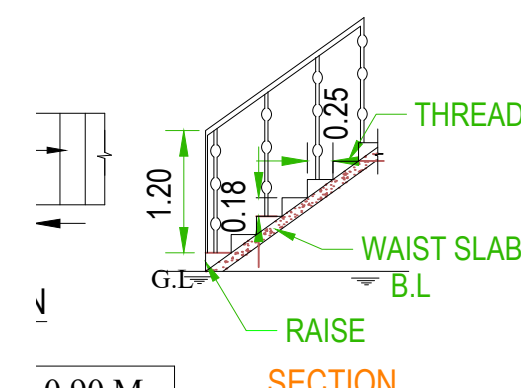
STAIRCASE DETAILS
