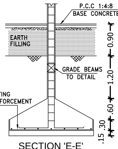
SECTION 'E-E'
