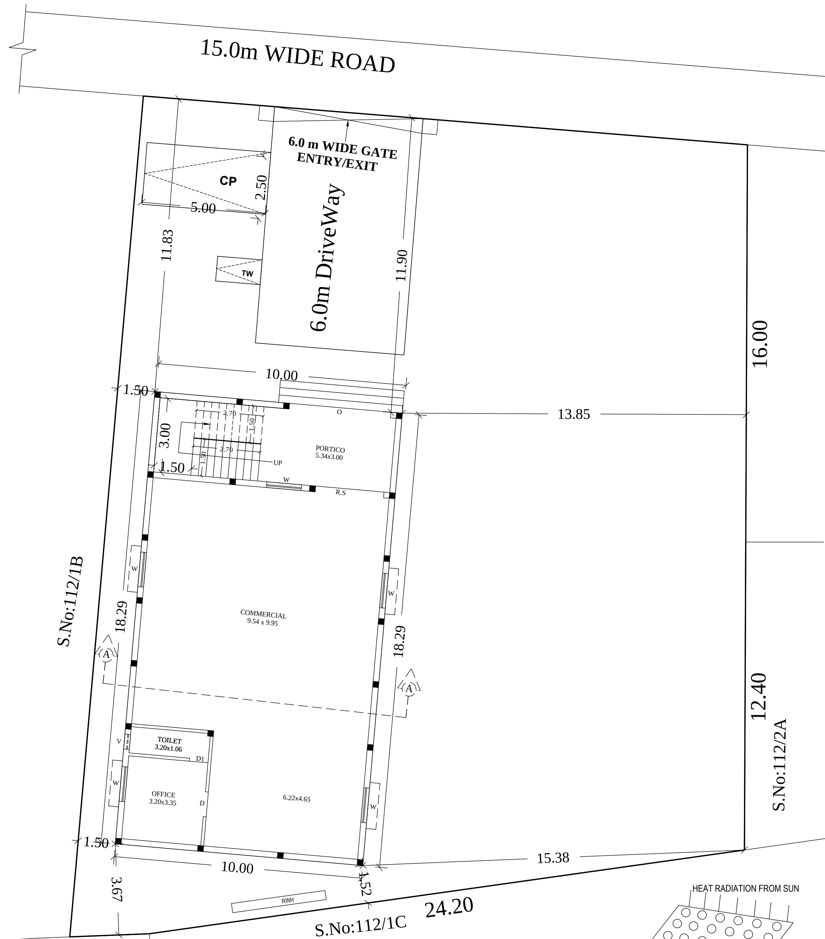
GE/PROPOSED GROUND FLOOR PLAN
