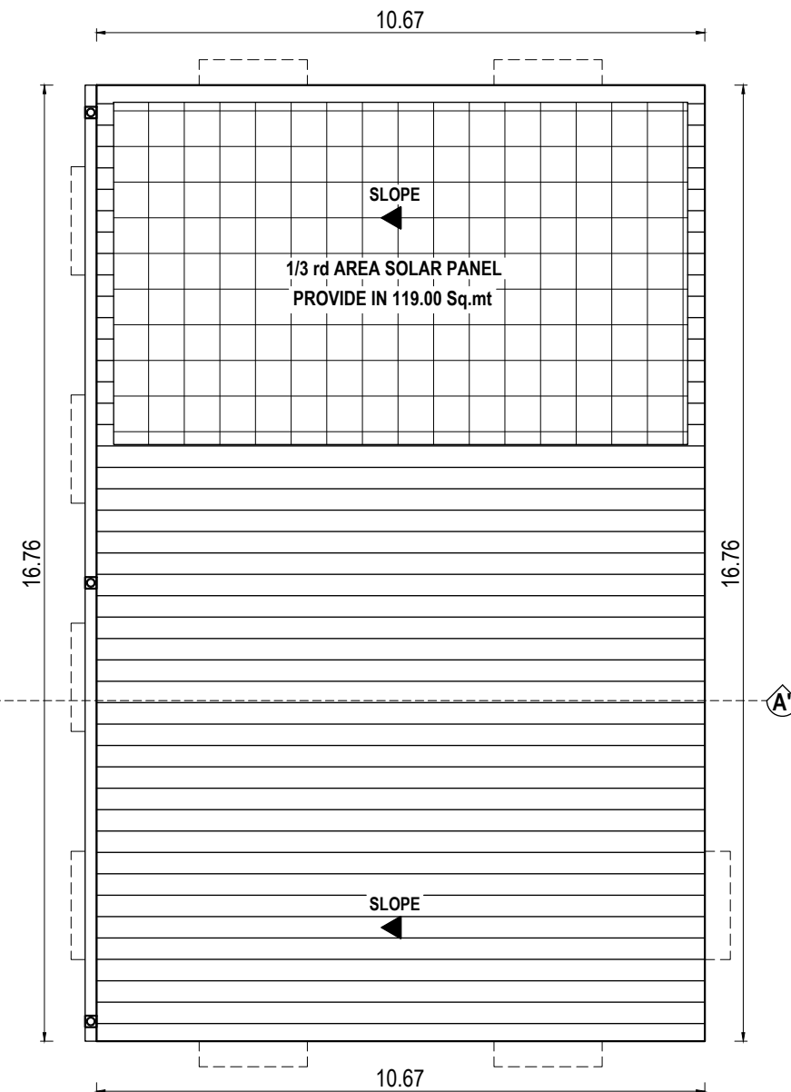
ROOF PLAN
