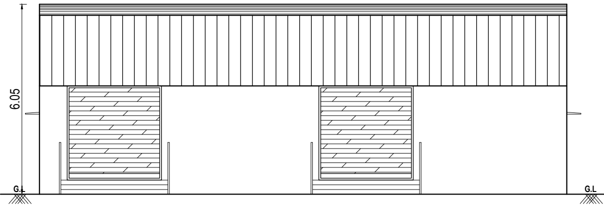
FRONT ELEVATION
