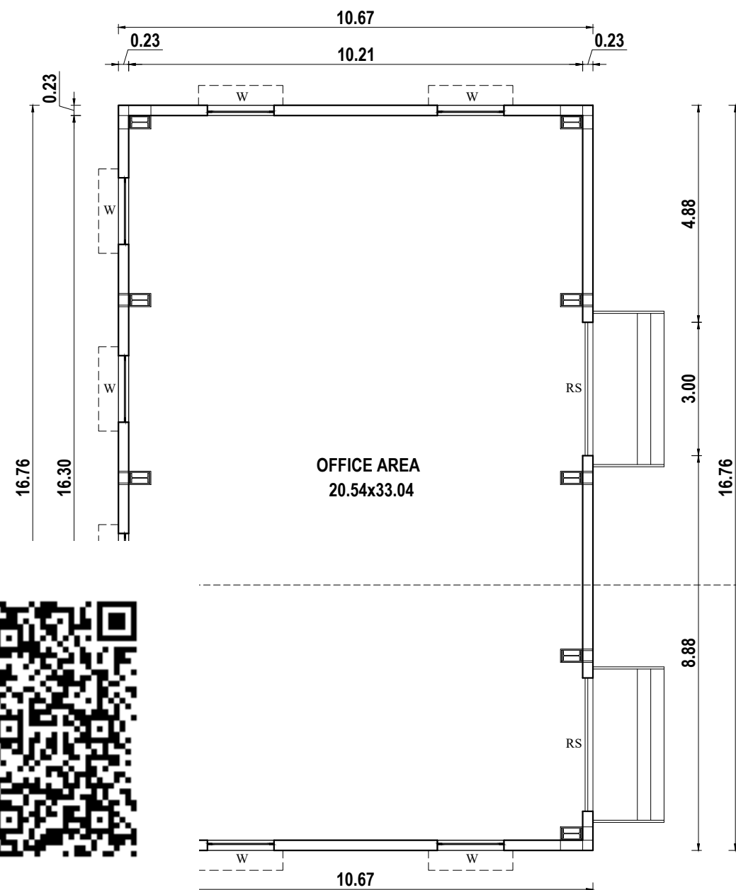
PROPOSED GROUND PLAN
