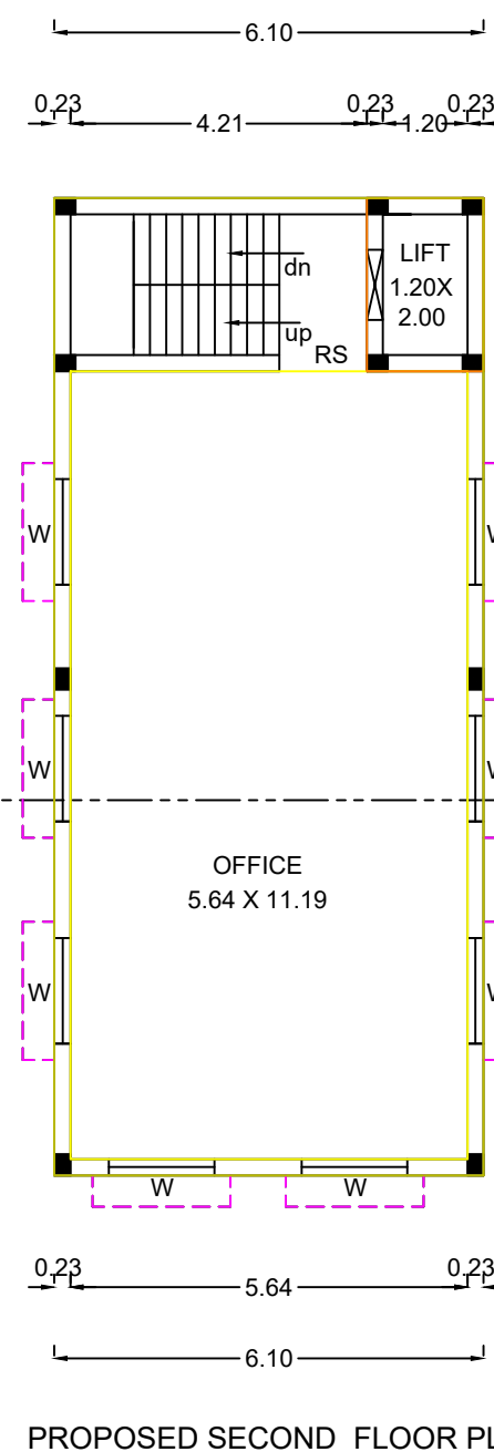
PROPOSED SECOND FLOOR PLAN
