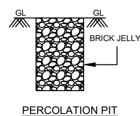
PERCOLATION PIT
