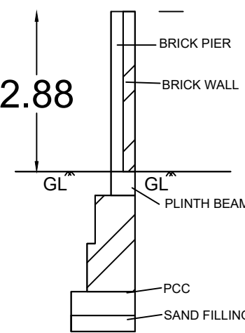
COMPOUND WALL
