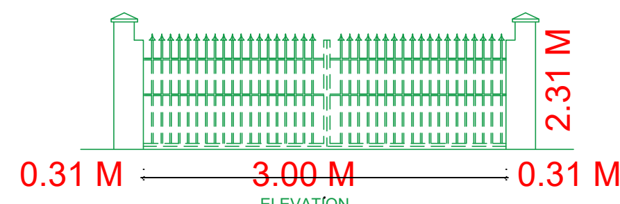
ELEVATION: GATE DETAIL
