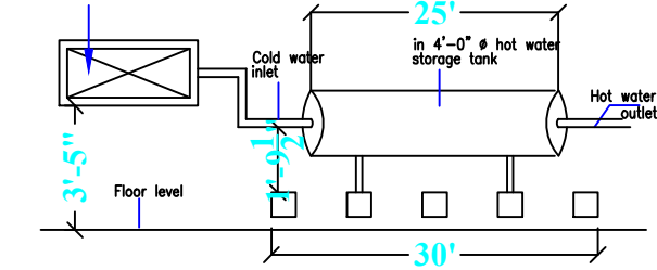
SOLAR HOT WATER SYSTEM(SWHS) DETAIL
