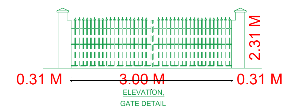
ELEVATION, GATE DETAIL
