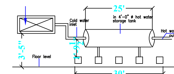
SOLAR HOT WATER SYSTEM(SWHS) DETAILS
