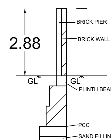
COMPOUND WALL
