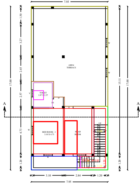
FIRST & TERRACE FLOOR PLAN
