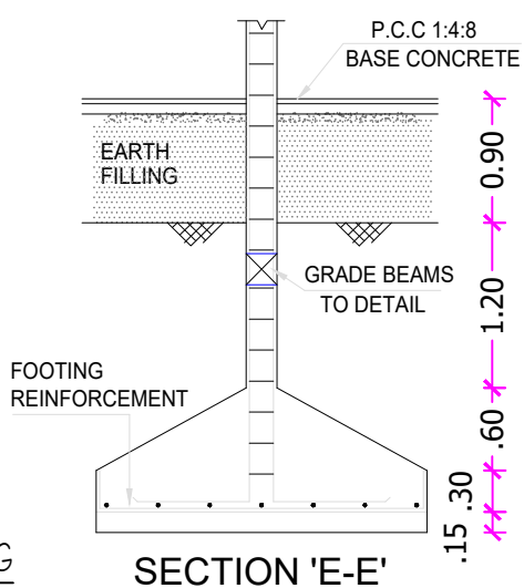
SECTION 'E-E'
