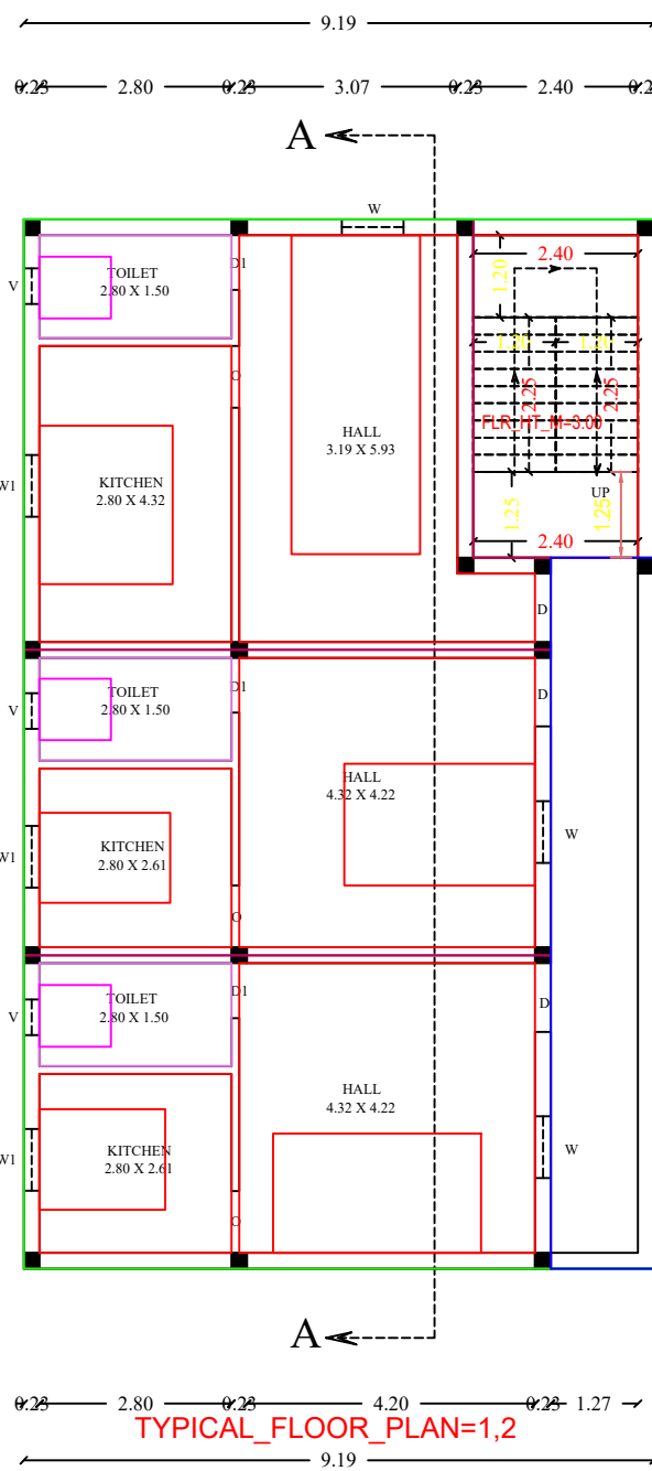
TYPICAL FIRST & SECOND FLOOR PLAN
