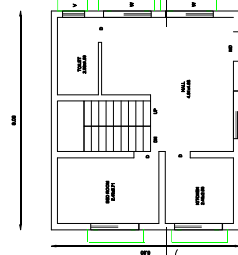
GROUND FLOOR
