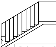
Staircase Details: Rise : 0.15m Tread: 0.25m Width : 1.0m Height : 1.25 m
