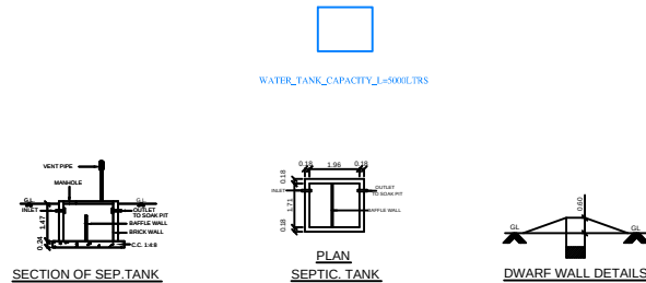
SECTION OF SEP.TANK
