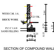
SECTION OF COMPOUND WALL
