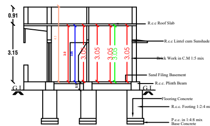
SECTION ON AA BLOCK 3
