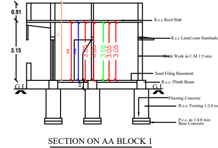
SECTION ON AA BLOCK 1
