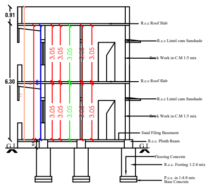
SECTION ON AA BLOCK 2
