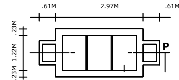
SEPTIC TANK PLAN
