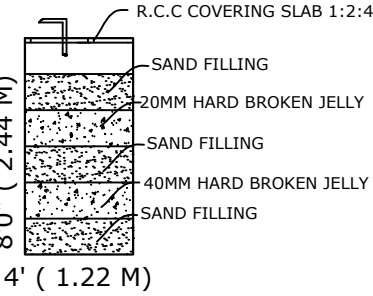
RAIN WATER 'H' UNIT
