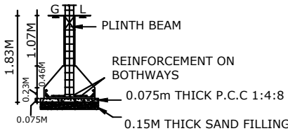
TYP. COLUMN FOOTING DETAIL
