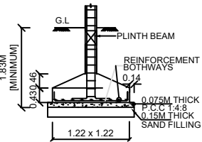
COLUMN FOOTING ( REFER STRUCTURAL DRAWING )
