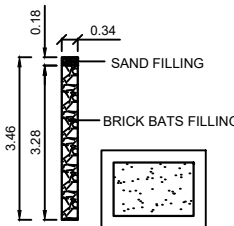
DETAILS OF PERCOLATION PIT
