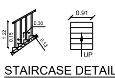
STAIRCASE DETAIL
