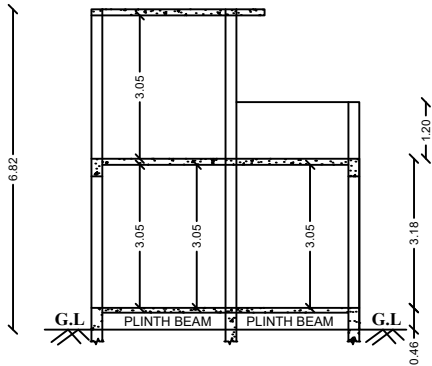
SECTION ON "A-L"
