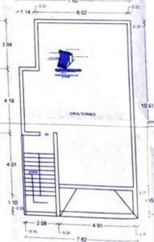
PROPOSED TERRACE FLOOR PLAN
